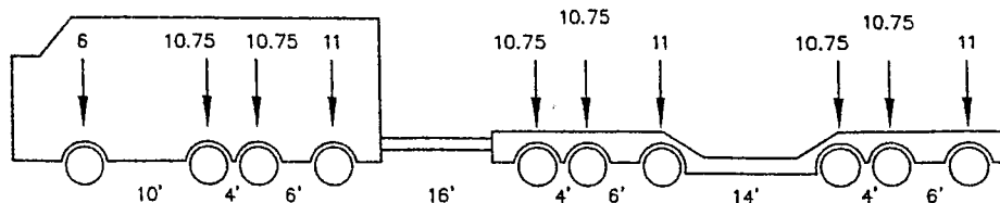
OVERLOAD 2 (103.5 TONS)
