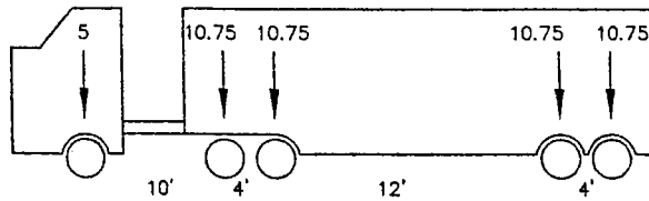
OVERLOAD 1 (48 TONS)
