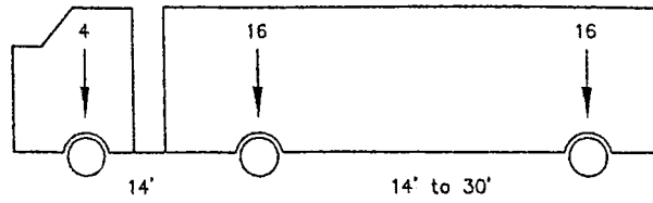
HS-20 (36 TONS)
