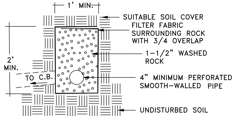
DRAIN DETAIL
