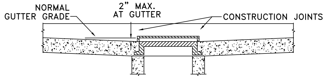
SECTION B-B
