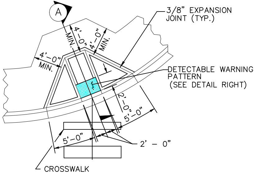
CURB RAMP TYPE 3 PLAN
