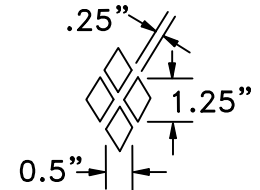
SURFACING TEXTURE DETAIL D
